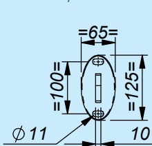
Top bracket
