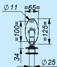
Bottom bracket
