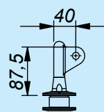
Gusset
