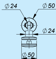
Bottom bracket
