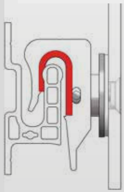
Hook system « free point » with anti-noise solution to avoid any noise pollution.
