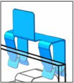
OPTION : the clip anti-translation ( Seismic zone, negative slope, extreme wind pressure )
